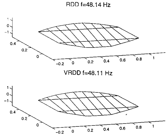
Figure 6: First rotational mode of mid span. Estimated by RDD and VRDD
