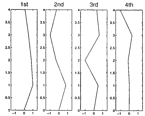
Figure 1: Mode shapes of 4 DOF system.
