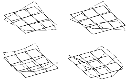
Figure 7. Upper left: Harmonic 304 Hz. Upper right: 1 st mode 368 Hz. Lower left: 2 nd mode 480 Hz. Lower right: 3 rd mode 704 Hz.
