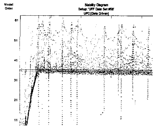
Figure 6 Stabilisation diagram
