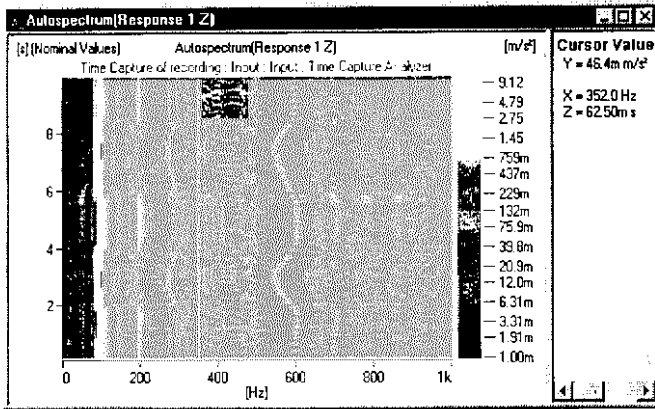
Figure 3 Contour plot from a narrow variation of the motor speed
