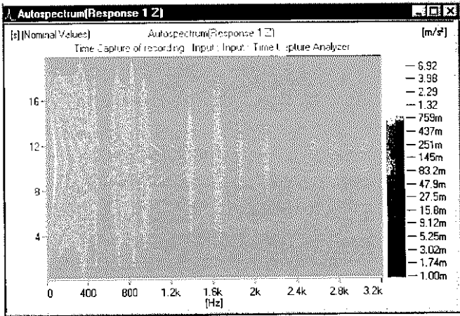
Figure 2 Contour plot from a broad run up/down
