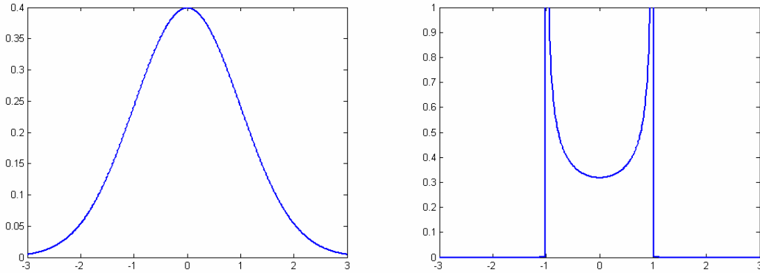
Figure 3. Normalized PDF of the response of a pure structural mode (left) and pure harmonic component (right)
